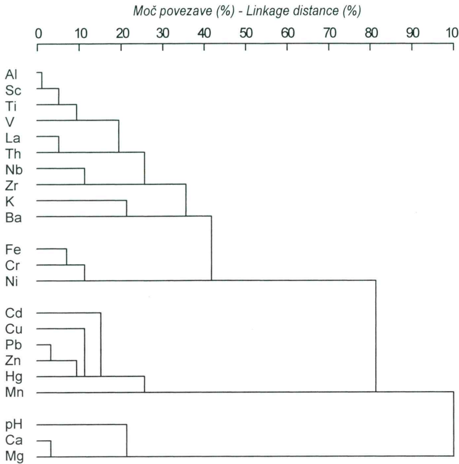
Fig. 3. Dendrogram of cluster analysis; n = 122 Sl. 3. Dendrogram clusterske analize; n = 122
