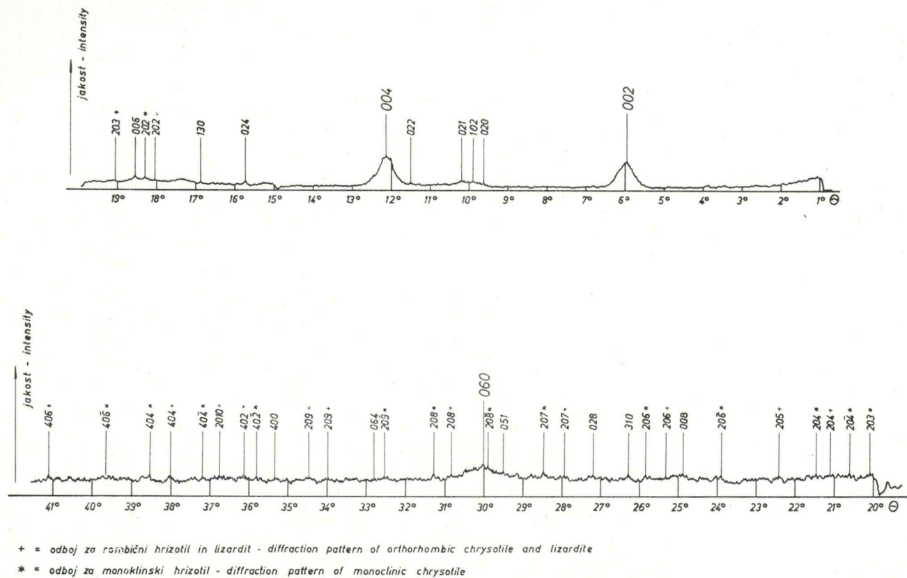
5. sl. Röntgenogram azbesta Stragari Fig. 5. X-rays diffraction pattern of the Stragari asbestos
