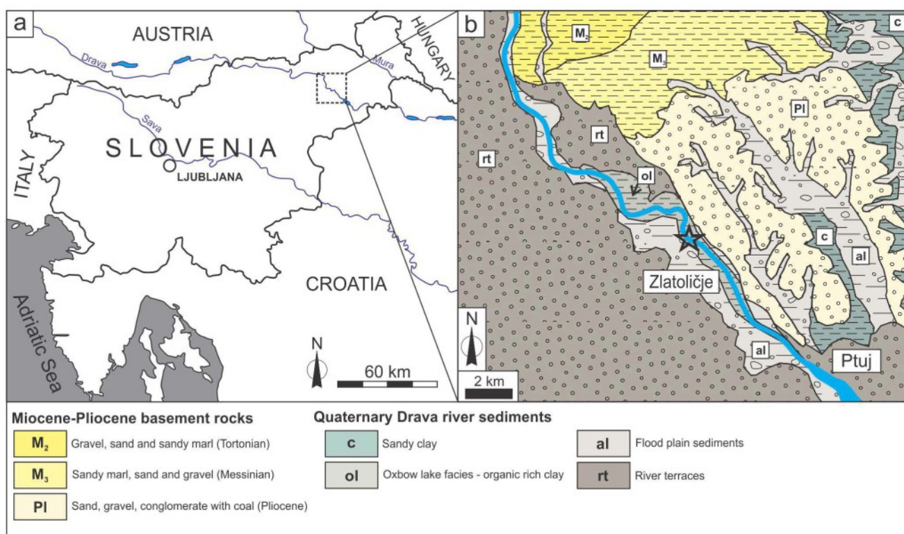
Fig. 1. Location of the study area (a) with detailed geological setting (b) (modified after ŽNIDARČIČ & MIOČ, 1987).
