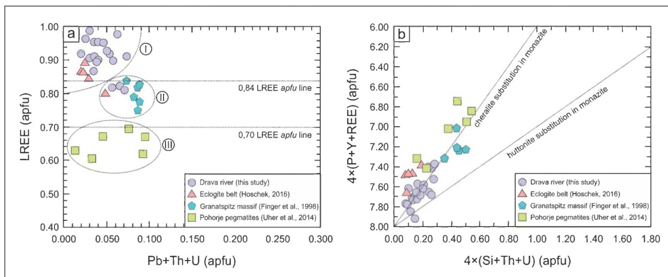
Fig. 6. Comparison of chemical composition (a) and the degree of isomorphic replacement in monazite (b) between studied Drava river monazites and monazites from Tauern Window and Pohorje Mts.
