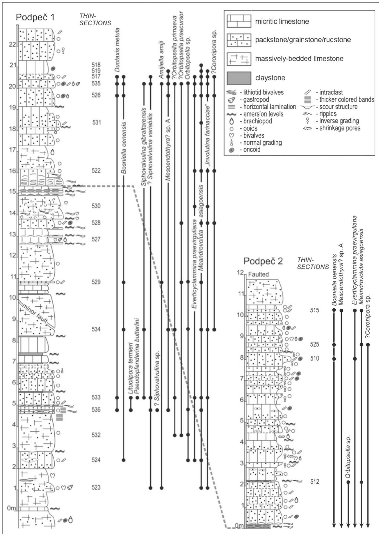
Fig. 3. Podpeč sections with distribution of foraminifera.
