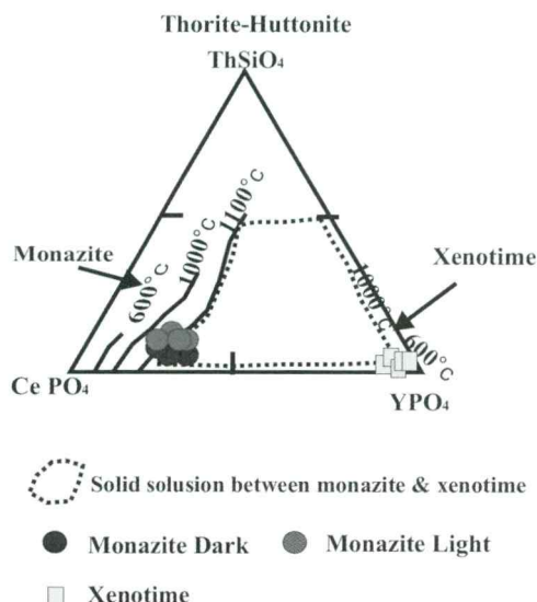
Fig. 8. Compositions of monazite and xenotime plotted in the \text{CePO}_4 - \text{ThSiO}_4 - \text{YPO}_4 ternary diagram (after GRATZ & HEINRICH, 1997). Dashed lines represent monazite compositions at the respective temperatures at 200 MPa (SEYDOUX-GUILLAUME et al., 2002).
