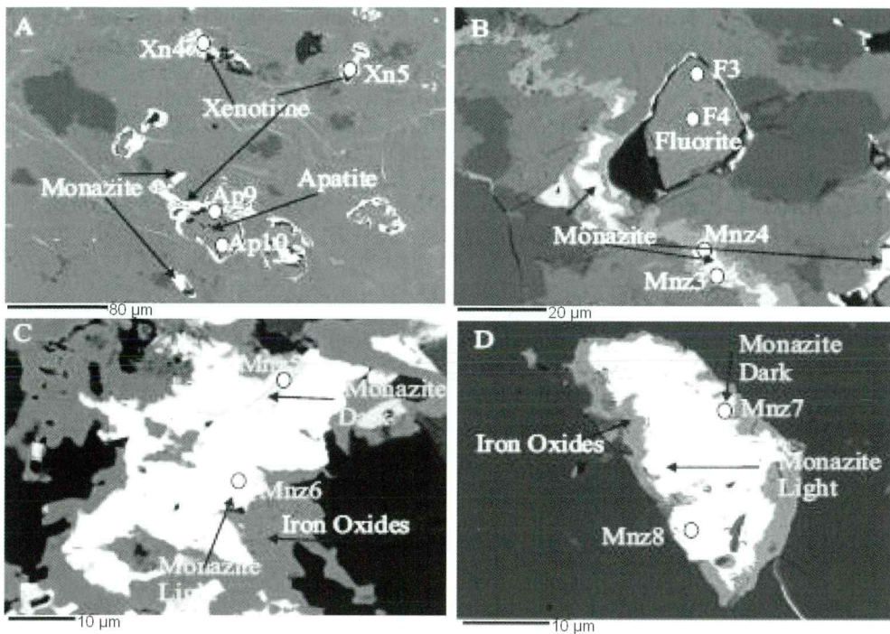
Fig. 5. SEM-BSE images of a) apatite altered and broken down to xenotime and monazite on the rim of apatite b) fluorite rimmed by monazite and xenotime on a rim, c) and d) heterogeneous monazite grain with darker and lighter parts, associated with iron oxides.
