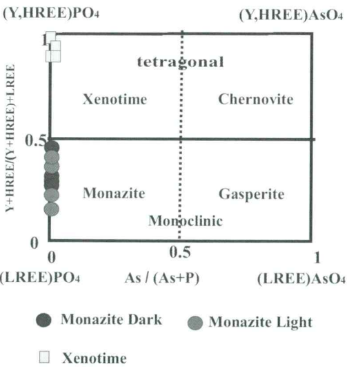
Fig. 7. Compositions of monazite-gasparite and xenotime-cheronovite solid solutions in quadrilateral classification diagram of the (Y,REE)AsO 4 -(Y,REE)PO 4 system (after ONDREJKA et al., 2007).
