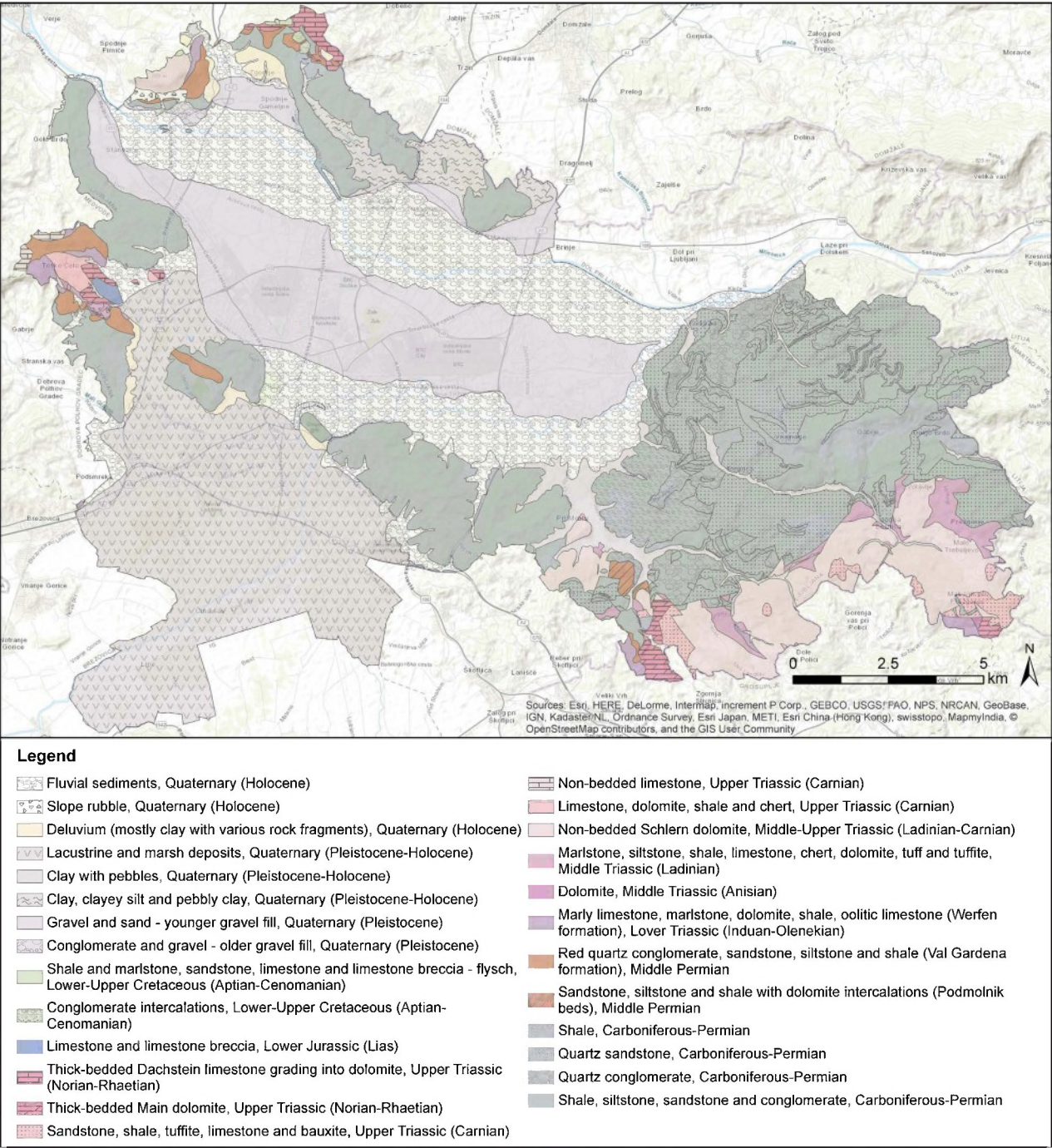
Fig. 6. The harmonized geological map of the study area.
