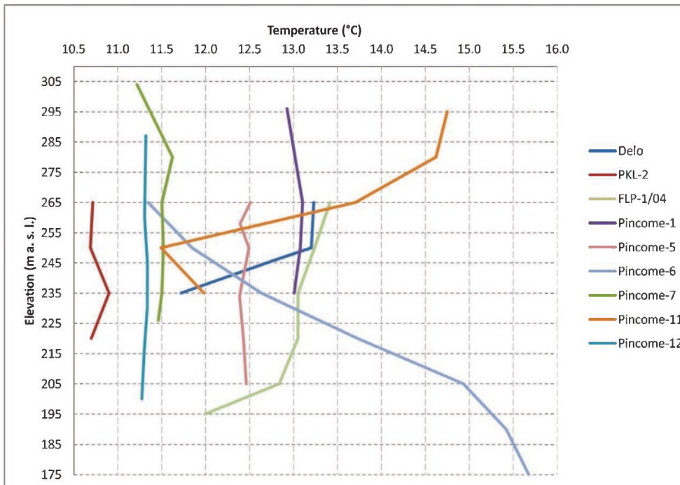
Fig. 12. Multi-level groundwater temperatures in observation wells.
