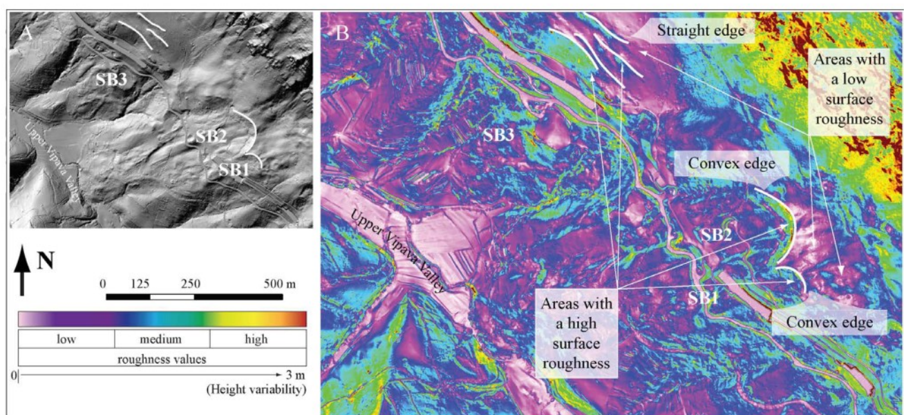
Fig. 4. (A) Shaded, digital terrain models (DTMs) with a resolution of 1 x 1 m, obtained by airborne laser scanning in the areas of SB1, SB2 and SB3 indicating the location of the convex and straight scarps. (B) A height variability map with the convex and straight scarps marked on SB1, SB2 and SB3. The upper arrows indicate an individual area with a very low surface roughness attributed to planation surfaces and the lower arrows indicate areas with high surface roughness, which are bound to individual convex scarps.
