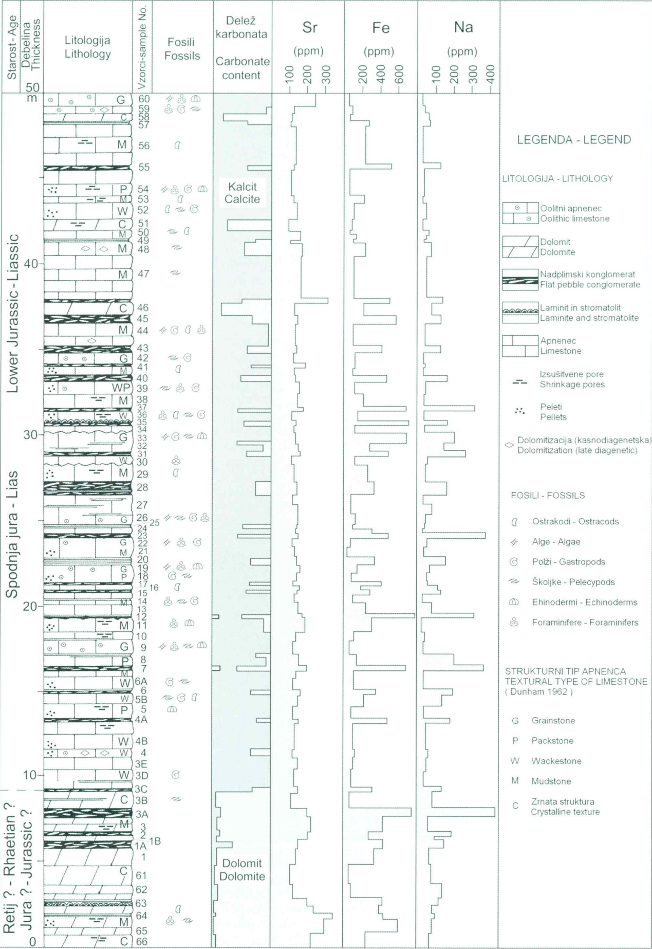
Sl. 2. Litologija in geokemija spodnje jurskih plasti v Preserju pri Borovnici Fig. 2. Lithology and geochemistry of Lower Jurassic beds in Preserje near Borovnica
