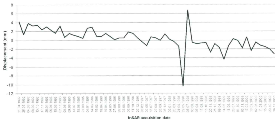
Fig. 13. Average displacements in millimetres for nine permanent scatterers from Fig. 12 relatively to the reference point. The post-earthquake surface equilibration is obvious.
