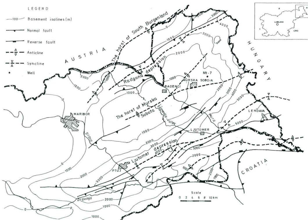
Fig. 1. Simplified tectonic map of the Mura basin (adapted from Ina-projekt OOUR KGI & Geološki zavod Ljubljana, TOZD GGG, 1986)
