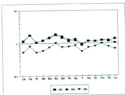
Fig. 2. PAAS normalised YREEs for the studied samples from Mt-7 well core (M1 – 925,20 m; M2 – 926,30 m; M3 – 1005,00 m)
