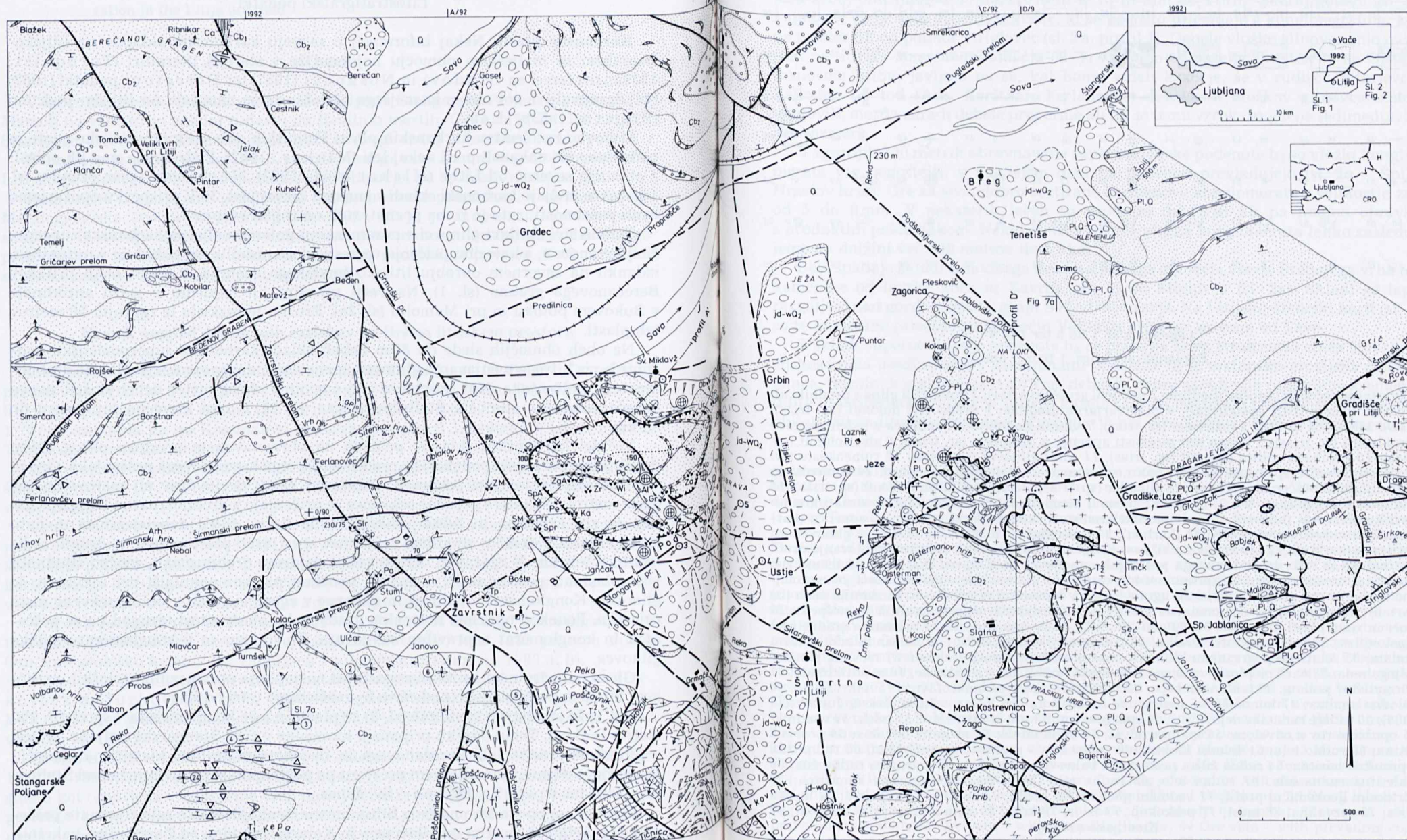
Fig. 1. Geological map of the Litija-Šmartno area
