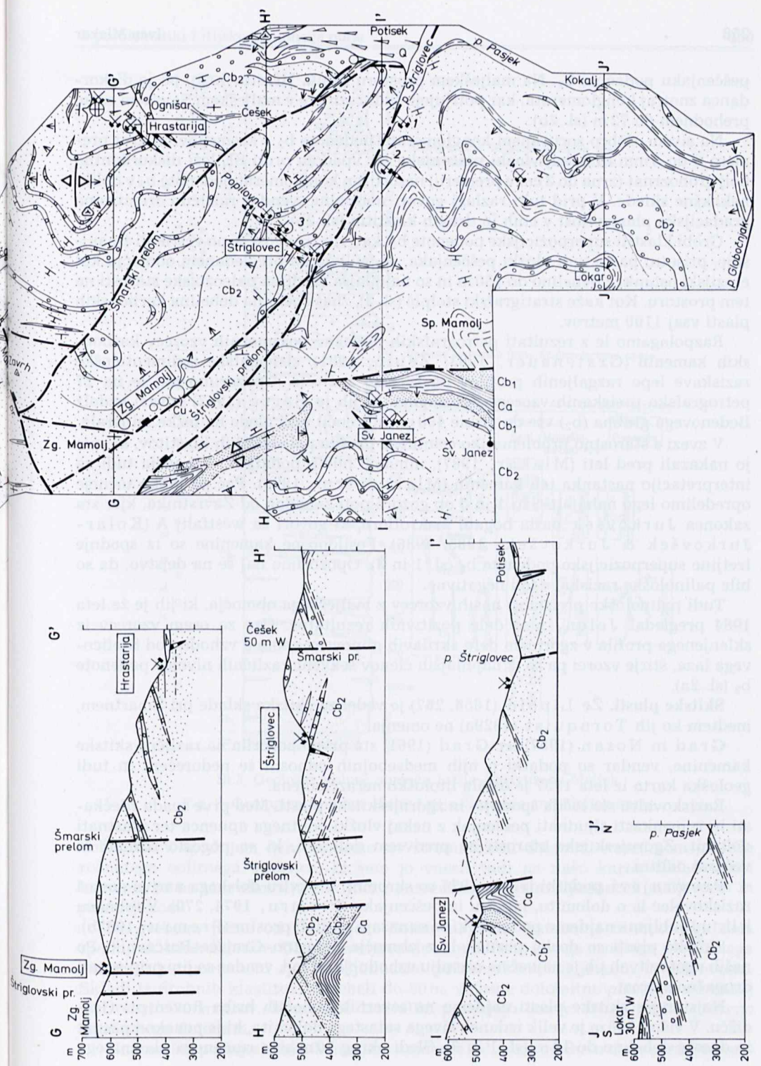
Fig. 2a. Maljek area – Geological map and geological cross sections Fig. 2b. Geology in the Sava adit (SR)
