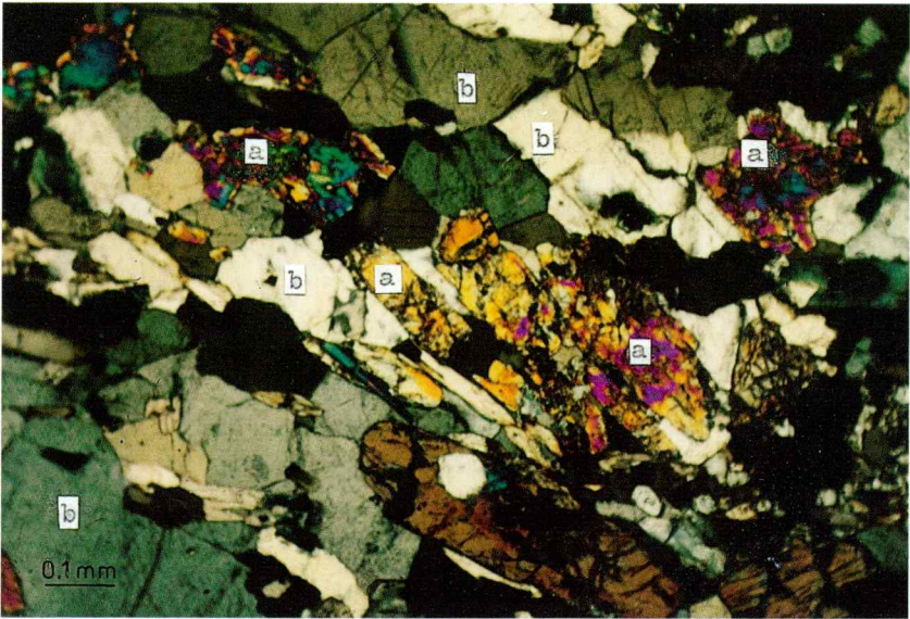
Fig. 2. Corroded and replaced Zn-rich aegirine-augite (a) relics by baryte (b) in baryte schists (N+, photo: S. Jančev)
