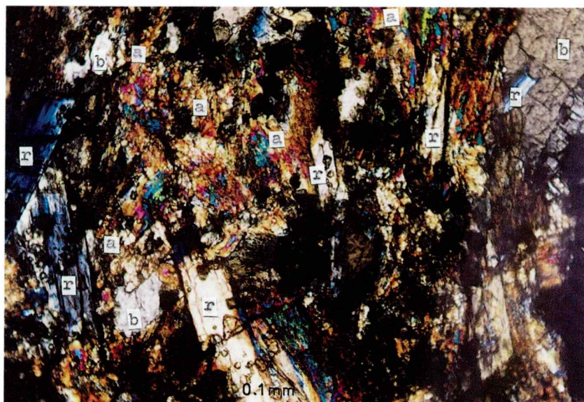
Fig. 5. Replacements of Zn-rich aegirine-augite (a) by Zn-rich richterite (r) inside of baryte (b) schist (N+, photo: S. Jančev)
