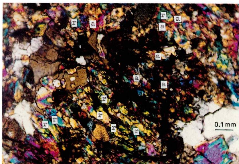
Fig. 6. Super fine-grained associations of Zn-rich aegirine-augite (a) replaced by Zn-rich richterite (r) fibres enclosed in dolomite marble (N+, photo: S. Jančev)
