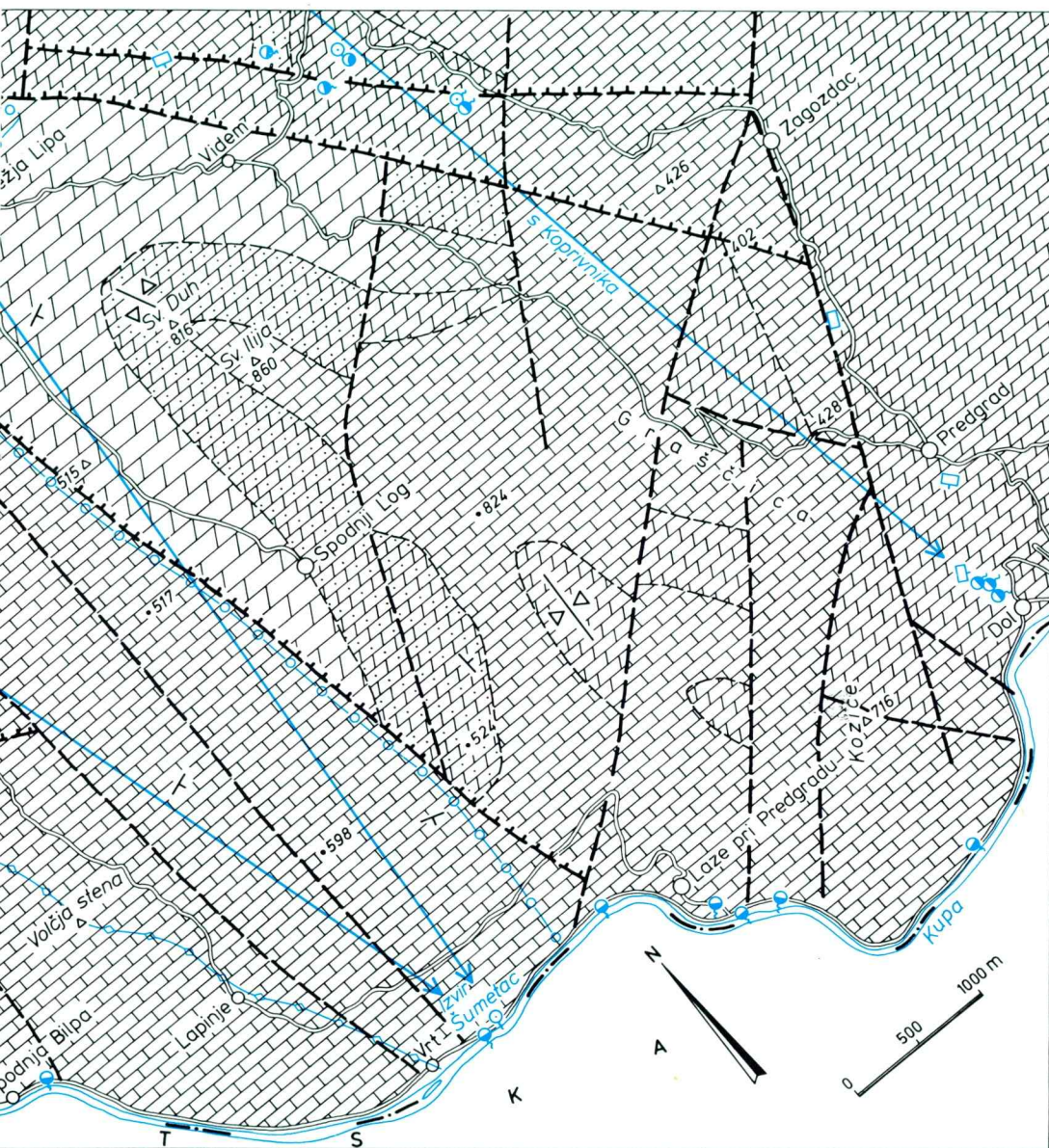
Fig. 1. Geological map of Šumetac area (Savić & Dozet, 1985)
