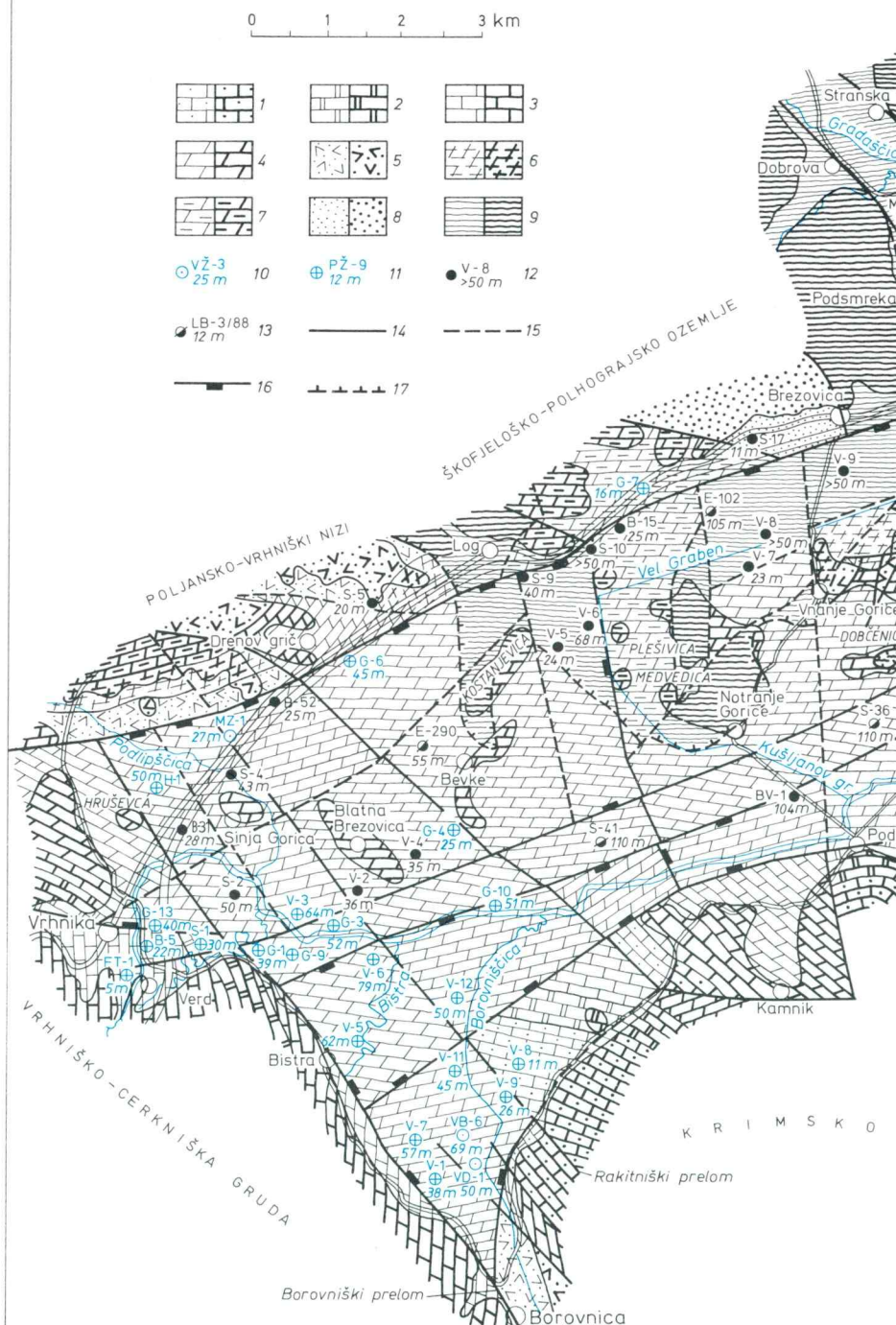
Fig. 2. Map of the Pre-Quaternary Basement of the Ljubljansko barje
