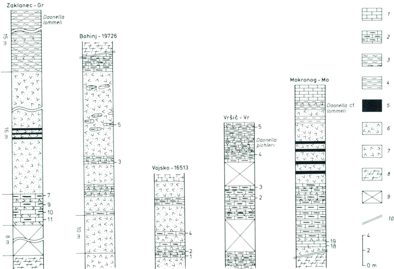
Fig. 2. Lithological columns of sections showing the position of radiolarian samples and co-occurring bivalves. The Zaklanec and Vršič sections are generalized according to Jurkovšek (1984) and Ramovš and Jurkovšek (1983 b) respectively
