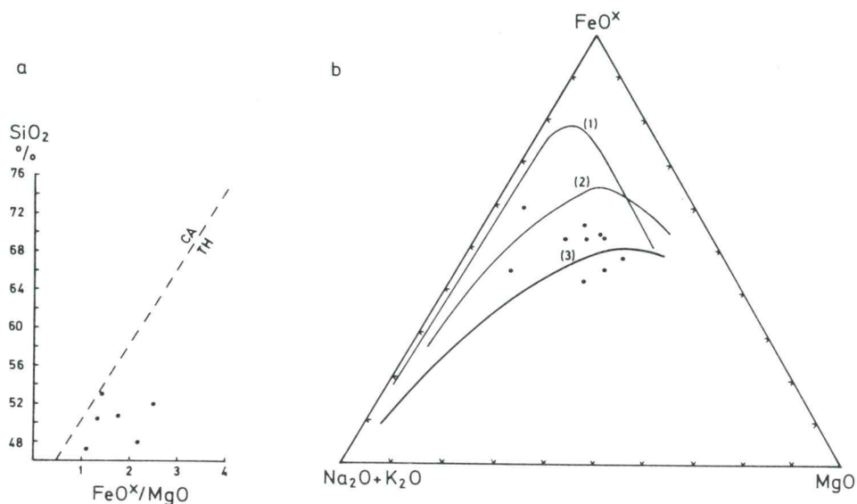
Sl. 2. a — Miyashirov dijagram \text{SiO}_2\text{:FeOx/MgO} , i b — trokomponentni dijagram \text{FeOx:Na}_2\text{O} + \text{K}_2\text{O:MgO}
