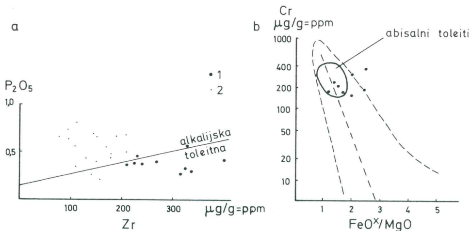
Sl. 3. a — dijagram \text{P}_2\text{O}_5\text{:Zr} , i b — dijagram \text{Cr:FeOx/MgO}
