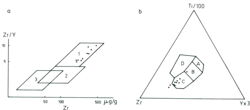
Sl. 6. a — dijagram \text{Zr}:\text{Zr}/\text{Y} i b — trokomponentni dijagram \text{Ti } 100:\text{Zr}:\text{Yx3}
