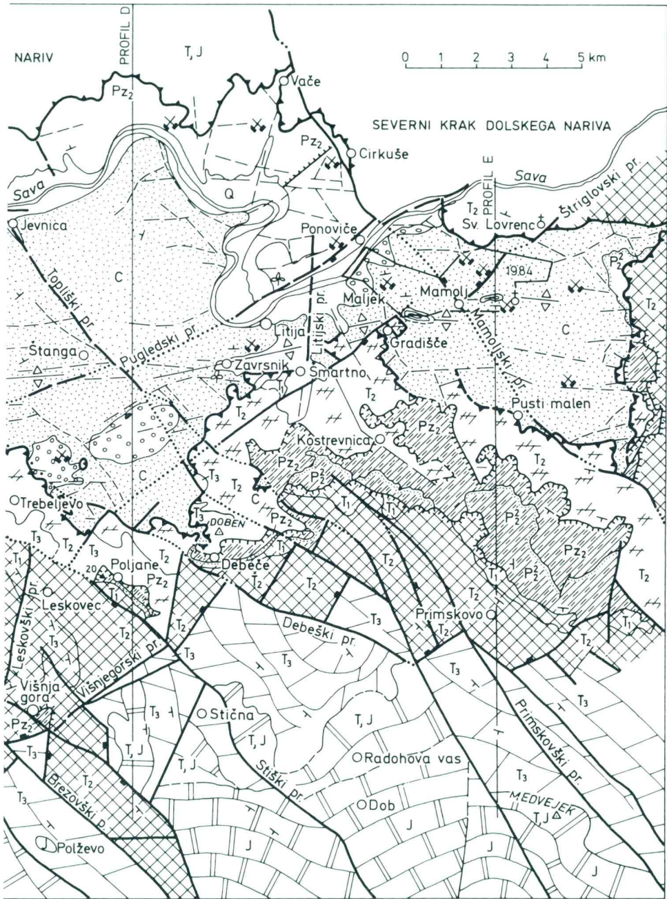
Fig. 1. Tectonic map of the Ljubljana-Litija region
