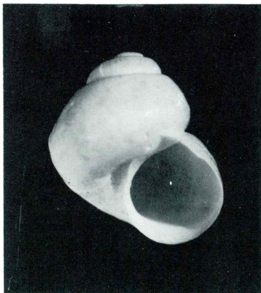
Sl. 2 — Fig. 2 Valvata (Cincinna) interposita Stefani, \times 15 Vrtina P-4up/78, globina 272 m Borehole P-4up/78, depth 272 m
