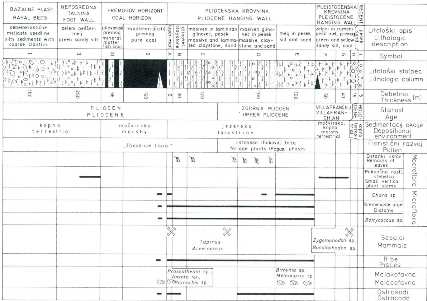
Sl. 9. Geološki stolpec s fosili Fig. 9. Geologic column with fossil remains
