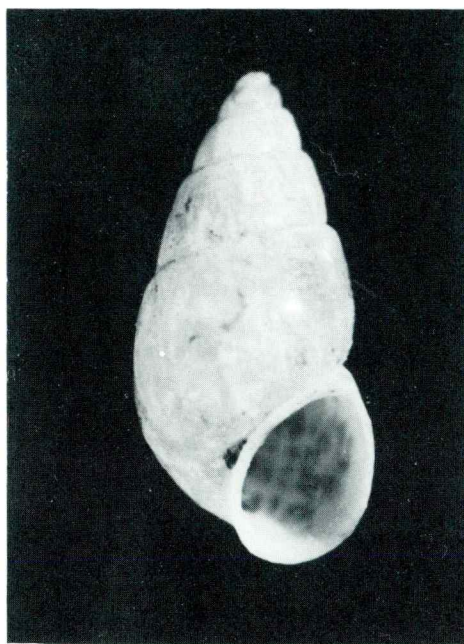
Sl. 3 — Fig. 3 Prososthenia ovata Bronn, \times 15 Vrtina P-4u/78, globina 274 m Borehole P-4u/78, depth 274 m
