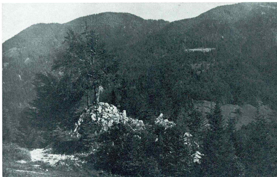
Sl. 4. Spodnja čer trogkofelskega apnenca pod žičnico Kranjska gora—Bedančev dom Fig. 4. The lower cliff of the Troglkofel limestone along the Kranjska Gora—Bedančev Dom aerial ropeway
