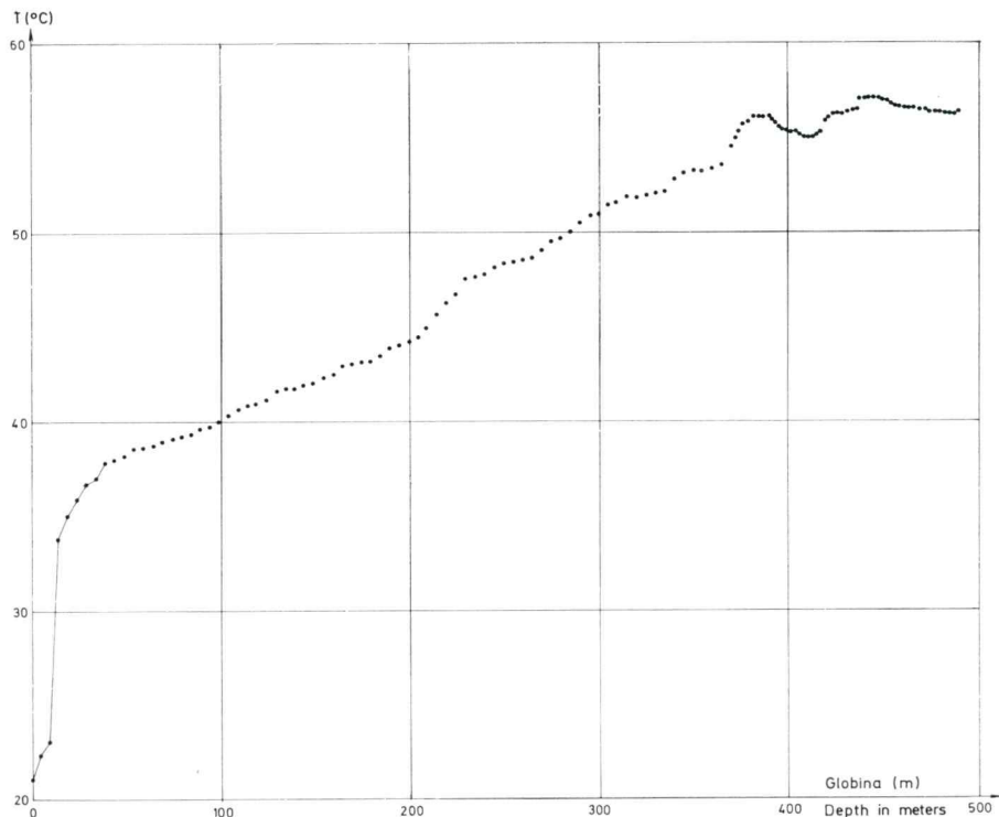
Sl. 1. Termogram vrtine V-10/71 Fig. 1. Temperature log of the bore hole V-10/71
