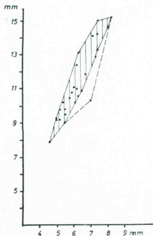
Fig. 1 a. Lymnaea peregra lagotis (Schränk); in vertical direction SH = thickness of shell; in horizontal direction VH = height of shell
