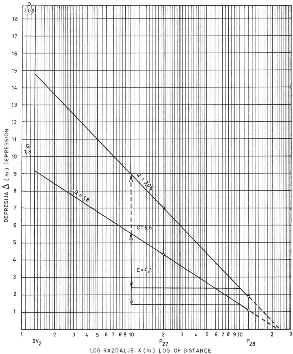
Sl. 6. Depresija v vrtini in piezometrih pri črpanju 1,8 \text{ m}^3/\text{h} in 3,06 \text{ m}^3/\text{h} Fig. 6. Depression of the water table in the drill hole located within the well BV_2 and piezometers at discharges 1,8 \text{ m}^3/\text{h} and 3,06 \text{ m}^3/\text{h}
