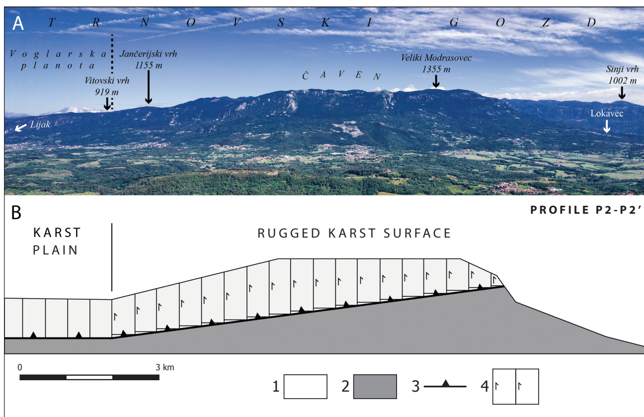
Fig. 5. Geomorphological profile P2 – P2': Voglarska planota (Voglari plateau) – Čaven (ridge) – Veliki Modrasovec (1355 m) – Lokavec (village). Position of profile in fig. 4.
