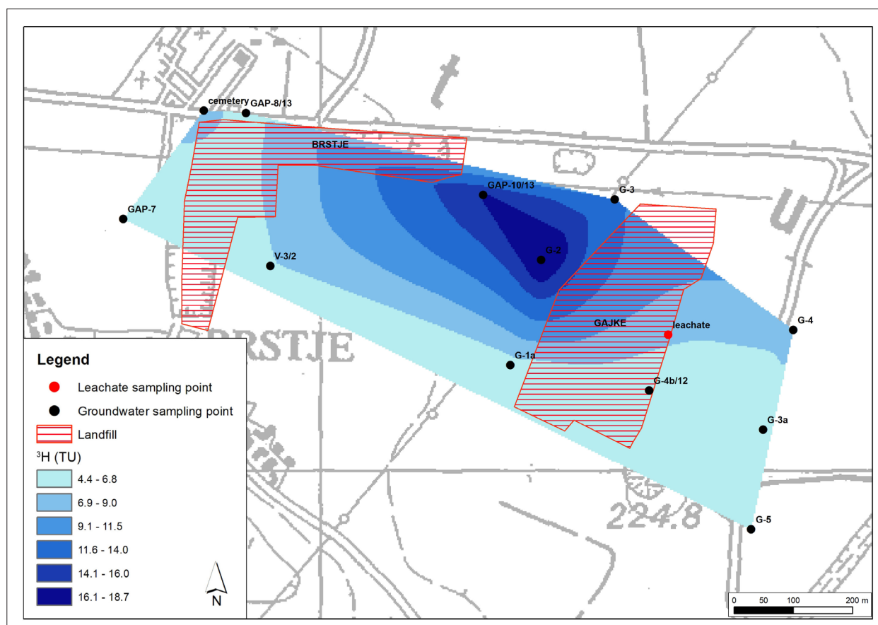
Fig. 9. Spatial distribution of ^3\text{H} (TU) in groundwater in the Gajke and Brstje landfill area.
