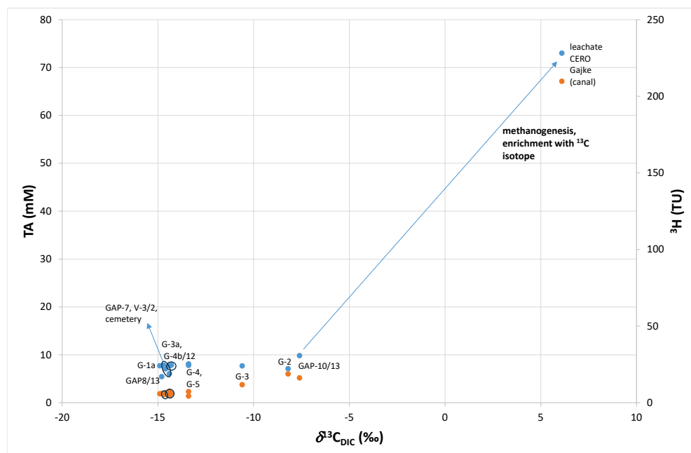
Fig. 8. TA and ^3\text{H} versus \delta^{13}\text{C}_{\text{DIC}} with associated locations.
