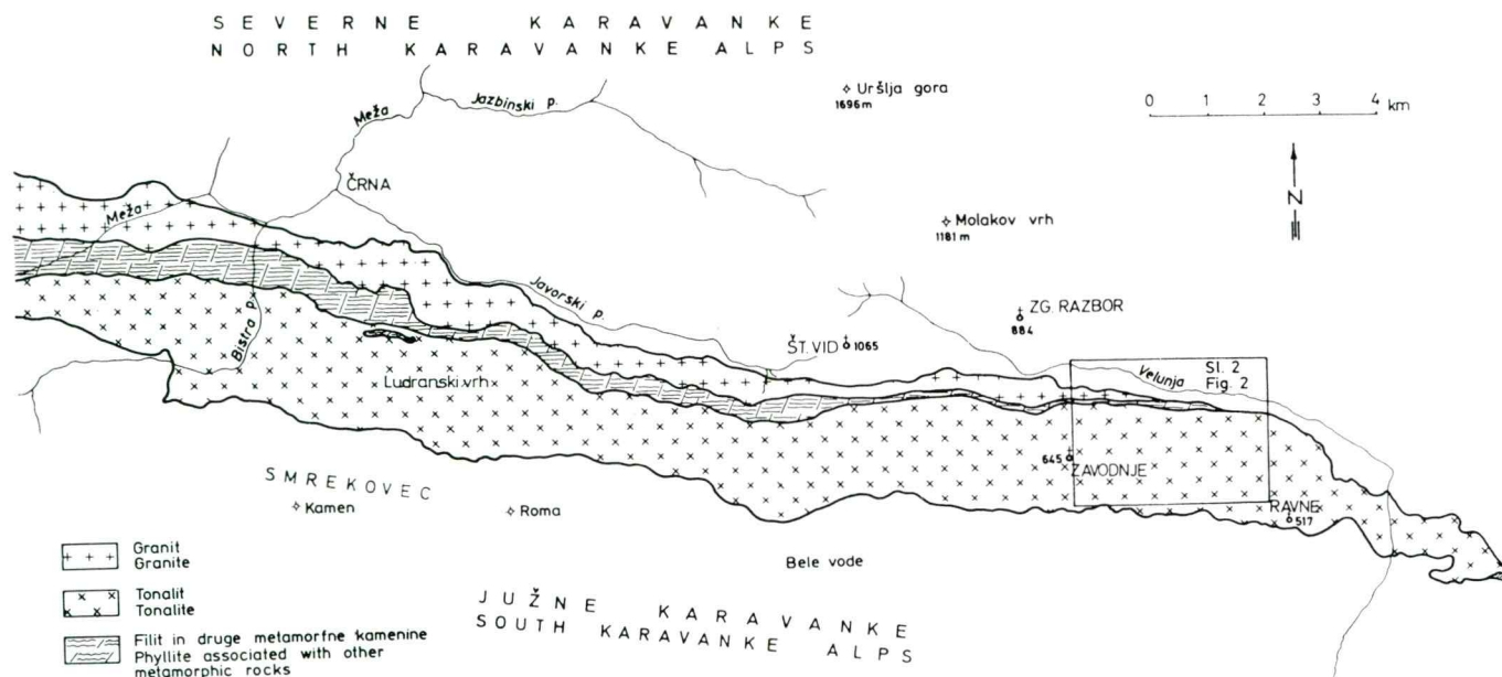
Fig. 1. Outline map of the Eisenkappel plutonic emplacement (according to F. Teller, 1896)
