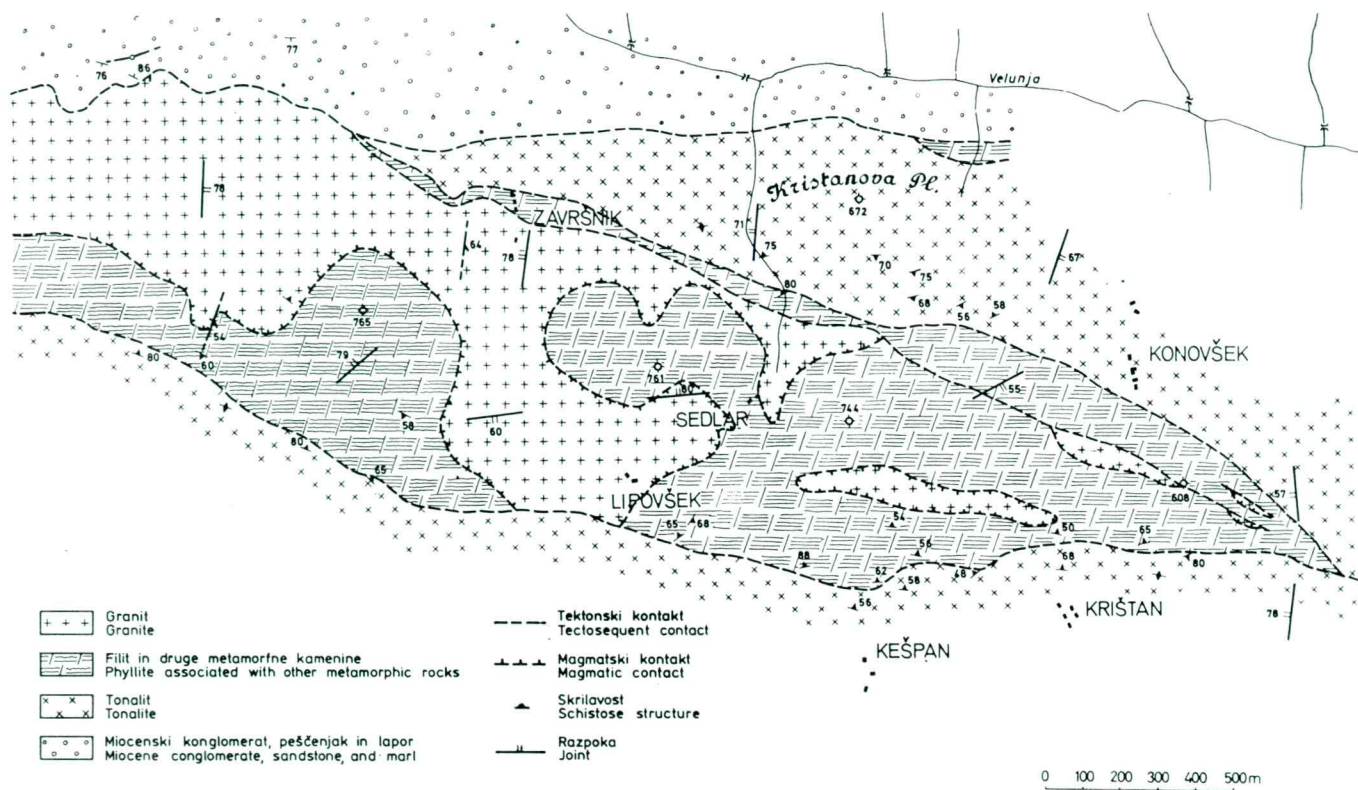
Fig. 2. Structural map of the eastern part of the Eisenkappel plutonic emplacement (according to S. Isailović & M. Miličević, 1964)
