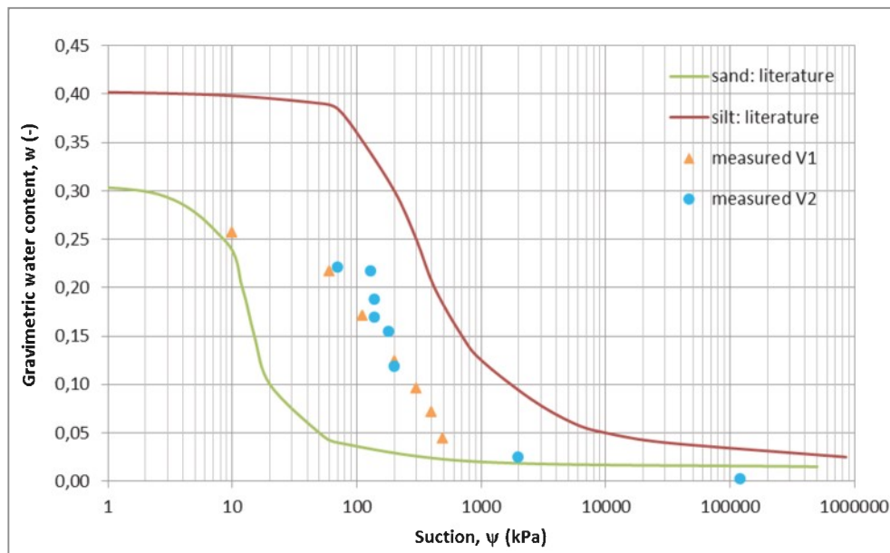
Fig. 7. Comparison of the measured values with data from the literature (the retention curves are according to FREDLUND et al., 2011).
