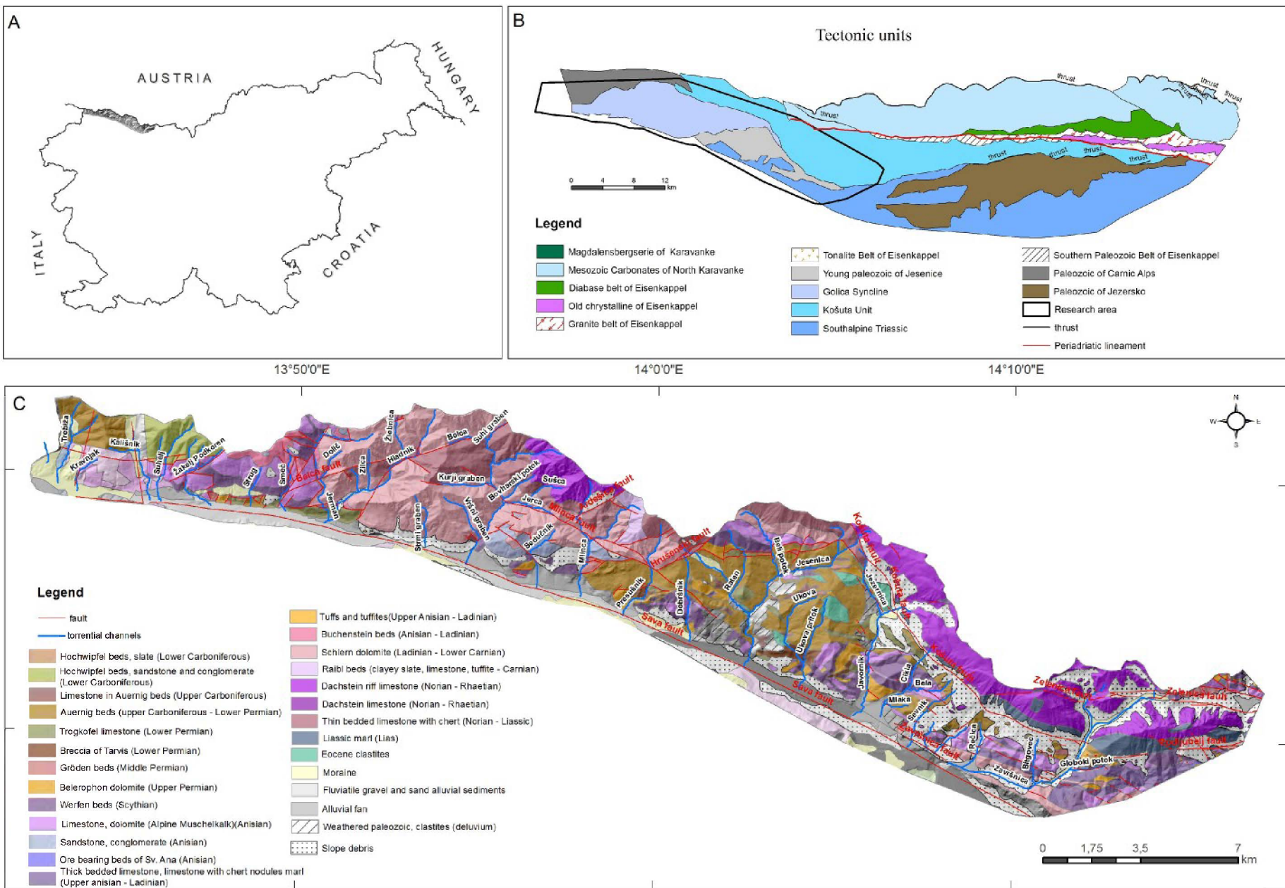
Fig. 2. Location of the Western Karavanke and the study area (modif. after BRENCIČ & POLJNIG, 2008). A. Geographic position; B. Tectonic Units of Karavanke; C. Geological map of western Karavanke (Slovenian part).
