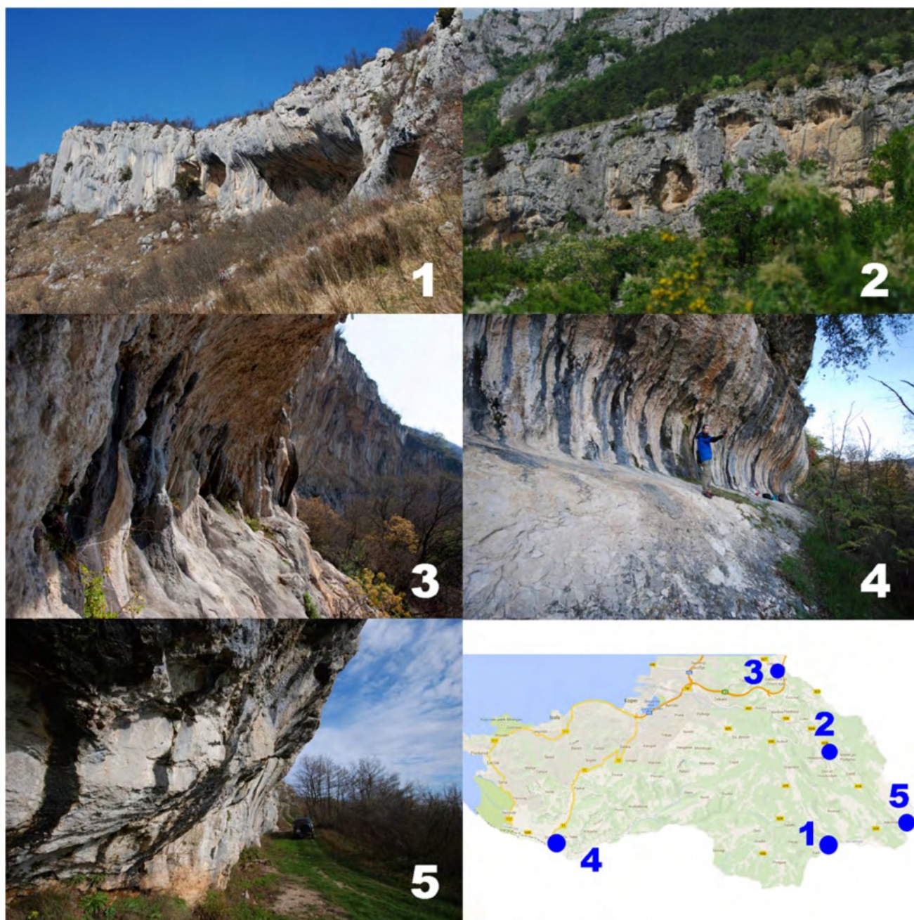
Fig. 1. Rock shelter locations, chosen for evaluation of geotourist potential: 1 – Veli Badin, 2 – Štrkljevisa, 3 – Mišja peč, 4 – Stena, 5 – Kavčič, and their position on the map showing the major part of Slovenian Istria. Author of the photos 1–5 (2012–2014): L. Ozis. Source of the map: Google maps, 2014.
