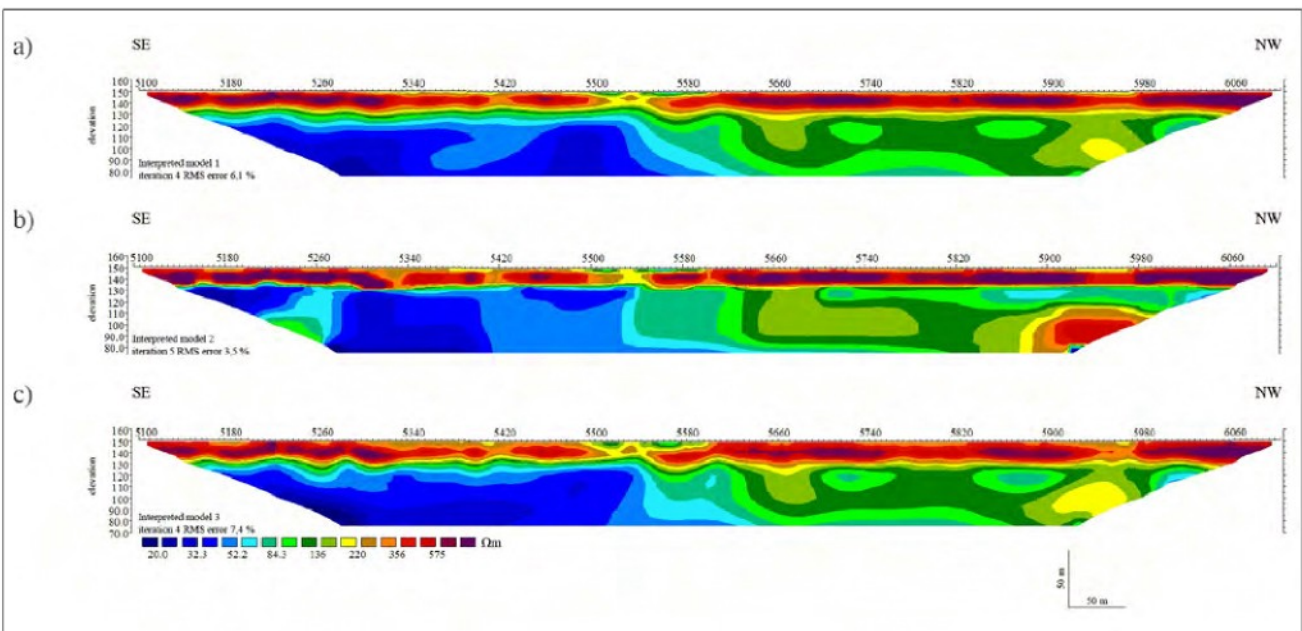
Fig. 9. Models created with RES2DINV: a) Model 1, b) Model 2 and c) Model 3. Sl. 9. Modeli izdelani s programom RES2DINV: a) model 1, b) model 2 in c) model 3.
