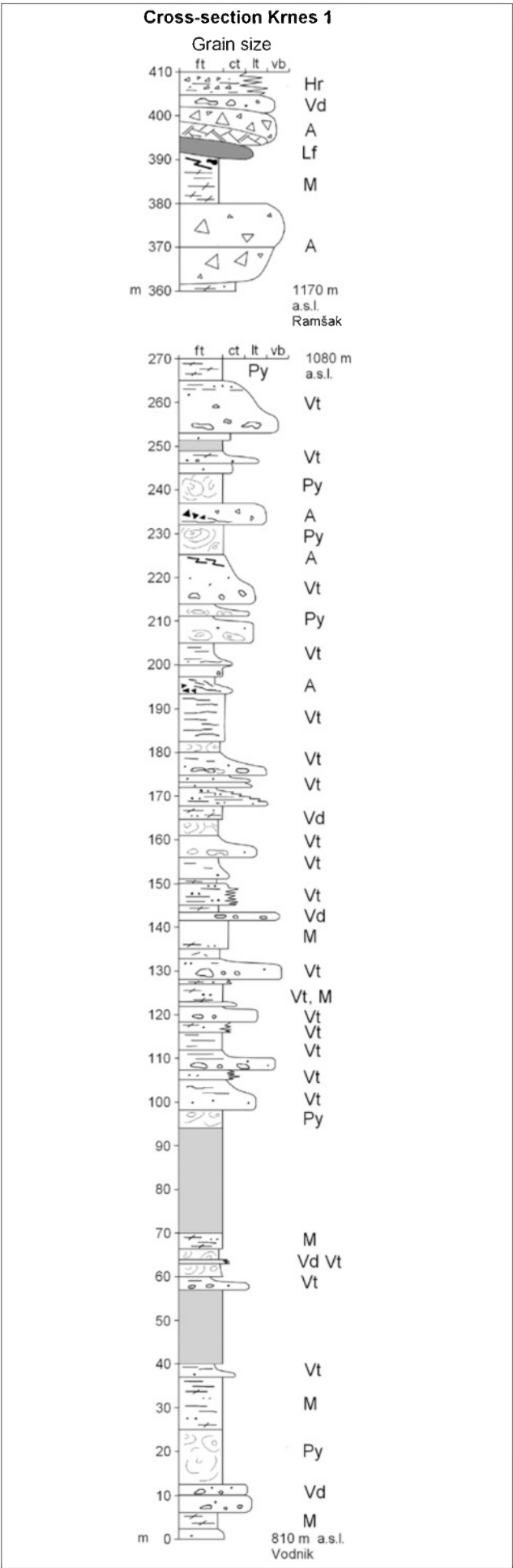
Fig. 5. Simplified cross-section Krnes 1 with the subsections Vodnik and Ramšak, the Smrekovec Volcanic Complex
