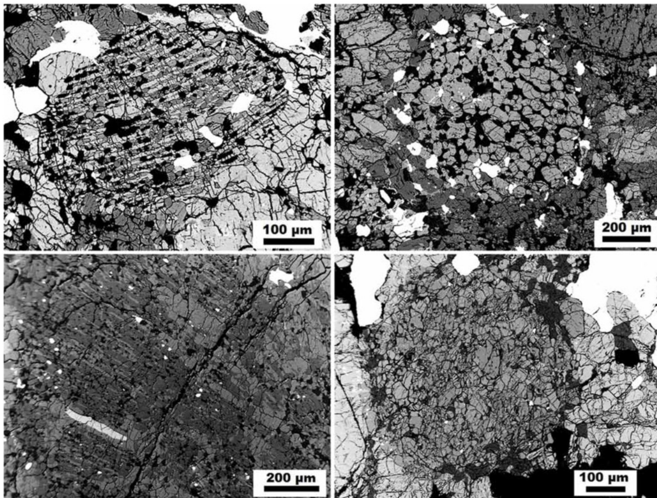
Fig. 3. Various types of chondrules in meteorite Jesenice. SEM, BSE. A) Barred olivine chondrule, B) Porphyritic olivine chondrule, C) Radial pyroxene chondrule, D) Porphyritic pyroxene chondrule
