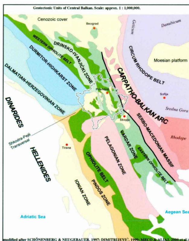
Fig. 1. Map of Kosovo in geotectonic units
