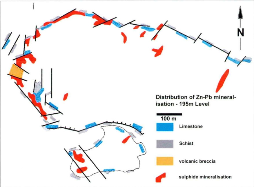
Fig. 5. Plan of 195 m level outline of anticline
