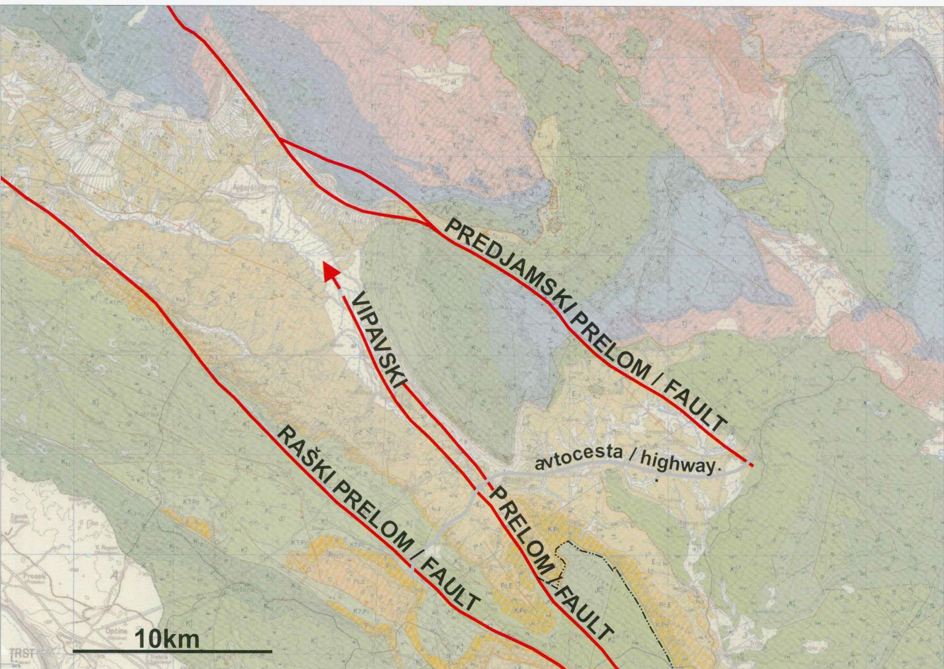
Slika 1. Geološka karta z vrisano prehojeno traso Vipavskega preloma (računalniška obdelava B. Celarc) Figure 1. Geologic map with course of the Vipava Fault verified in the field (computer treatment B. Celarc)
