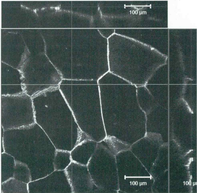
Slika 6. Posnetek toplotno staranega marmorja po 50 ciklu-sih ogrevanja in ohlajanja v temperaturnem razponu od 20 do ca. 60 °C. Na sliki je vidna jasna mreža razpok med zrn, ki se nadaljujejo tudi v globino (povečava objektivna 20x; 0,75 NA, globina posnetka je 82 µm) Figure 6. Image of thermally aged marble after 50 cycles of heating and cooling in temperature range of 20 to ca. 60 °C. Cracks which follows grain borders and progress into the stone structure can be clearly seen (objective magnification 20 times; 0.75 NA; depth of image is 82 µm)
