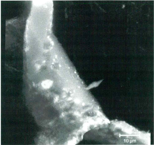
Slika 9. Detajl trans-granularne razpoke v toplotno staranem marmorju (oljni objektiv s povečavo 63 x; 1,4 NA) Figure 9. Detail of transgranular crack in thermally aged marble (oil objective, magnification 63 times; 1.4 NA)
