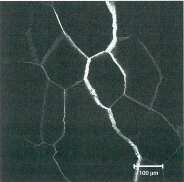
Slika 5. Mreža trans-granularnih razpok v toplotno staranem marmorju (povečava objektivna 20 x; 0,75 NA) Figure 5. Net of transgranular cracks in thermally aged marble (objective magnification 20 times; 0.75 NA)
