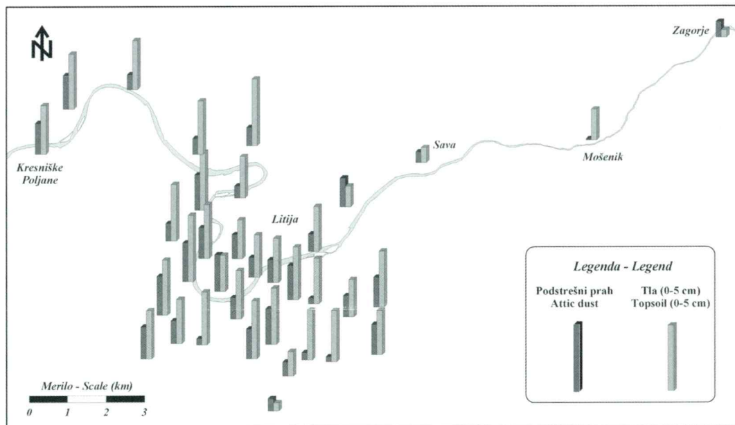
Slika 3. Prostorska porazdelitev faktorja 1 (Al, Co, Ce, K, La, Li, Nb, Rb, Sc, Ta, Th in Ti). Figure 3. Spatial distribution of factor 1 scores (Al, Co, Ce, K, La, Li, Nb, Rb, Sc, Ta, Th and Ti).
