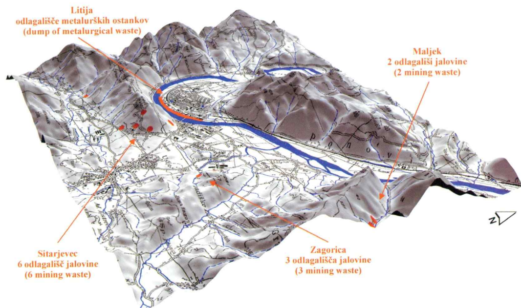
Slika 3. Lega odlagališč jalovine in metalurških žlinder Figure 3. Locations of mine and metallurgic waste deposits
