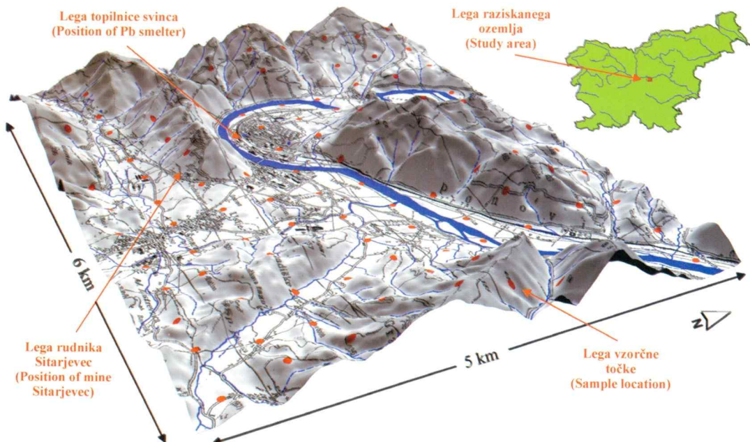
Slika 1. Lega raziskanega ozemlja z lokacijami vzorčenja Figure 1. Location of study area with sampling locations
