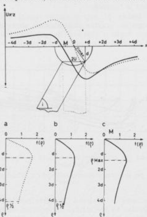
Fig. 4. Gravimetrical sounding above a vertical and an inclined dike of infinite depth extent
