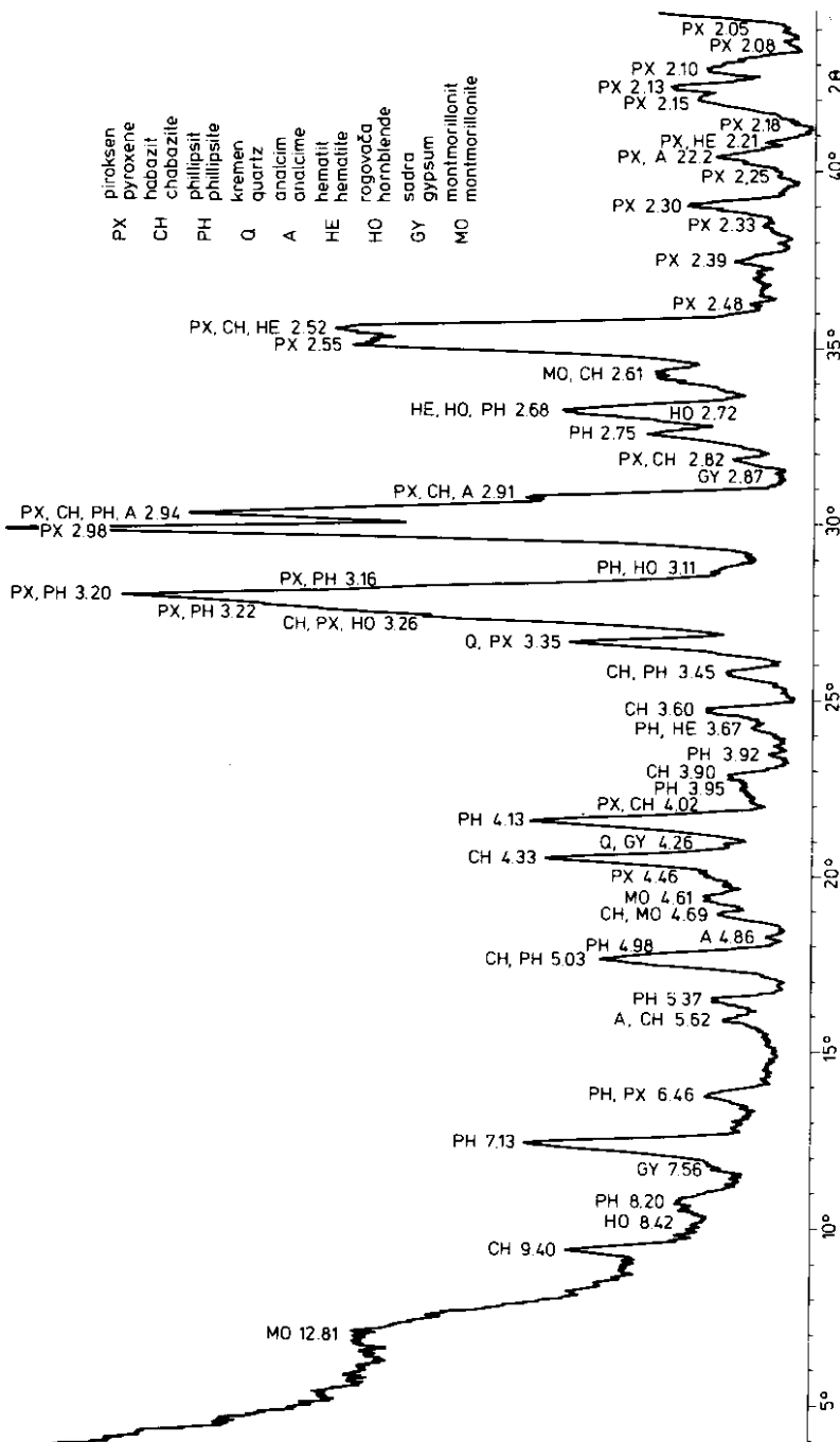
Sl. 2. Difraktogram vprašnega bazaltnega tufa Fig. 2. X-ray powder diffraction pattern of basaltic tuff
