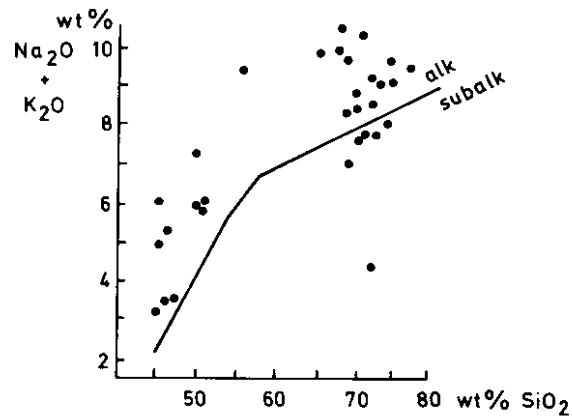
Sl. 4. Dijagram SiO 2 : Na 2 O + K 2 O (Miyashiro, 1974)
